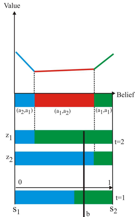
Figure 3.8: The two step value function for executing action a_1 as the initial action.
