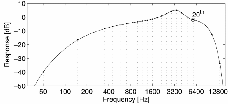
Figure 5.2. Outer and middle ear model according to Terhardt [43]
