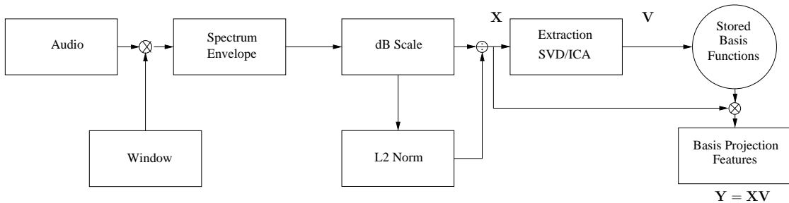
Figure 4.2. Computation of Spectral Bases and the projected features
