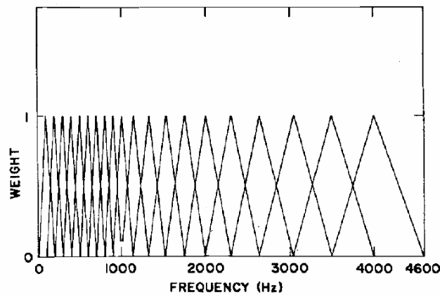
Figure 2.5. Filters for generating th Mel-scale Cepstral coefficients
