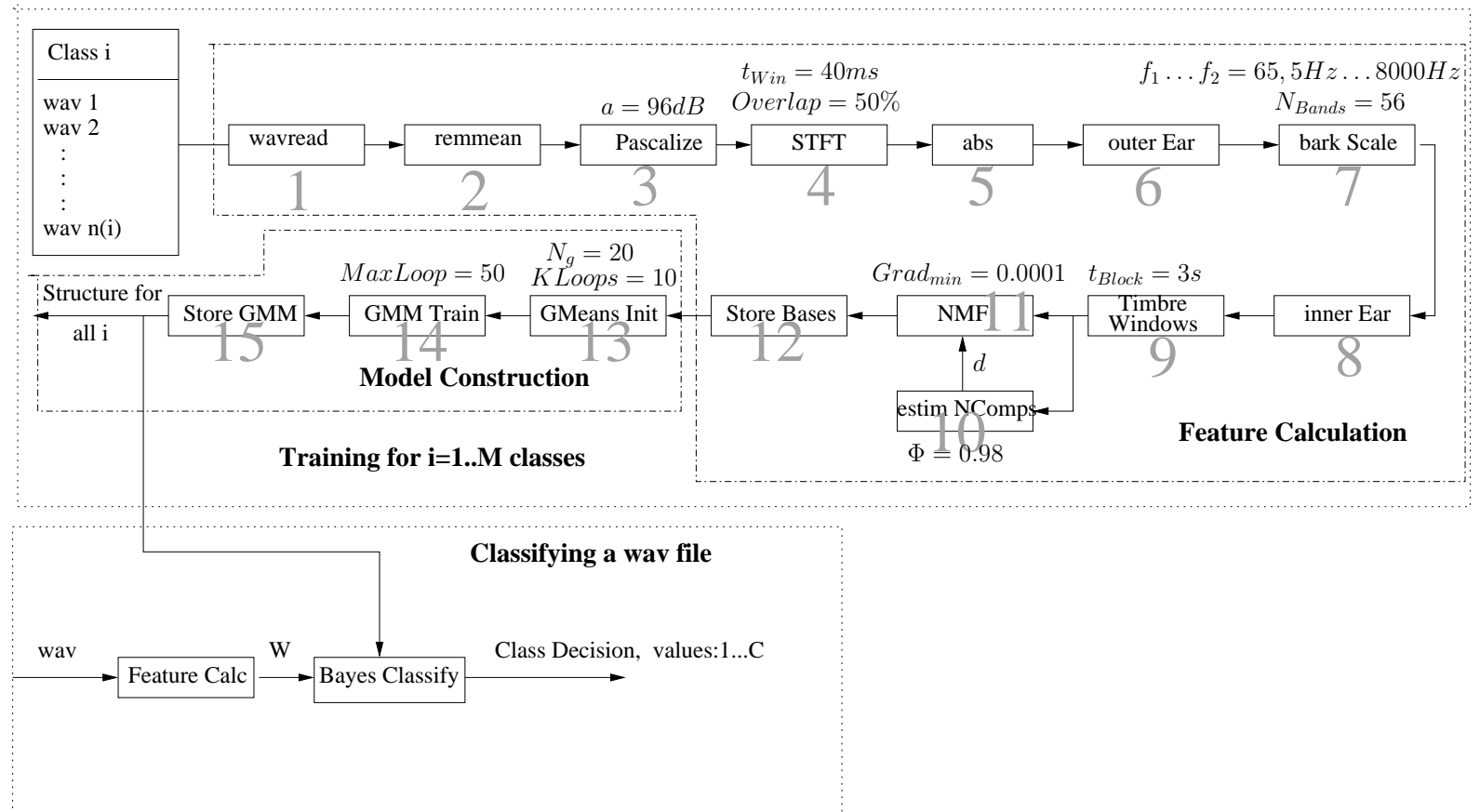
Figure 5.1. Initial concept for the Component Based Music Similarity System
