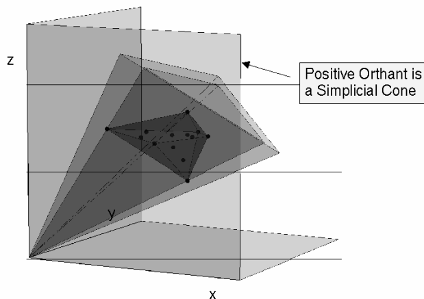
Figure 2.2. The columns of \mathbf{W} define a simplicial cone containing the columns of the approximated matrix, simplified example in three dimensions, from [14]
