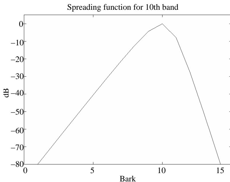
Figure 5.4. Spreading function for the 10th band
