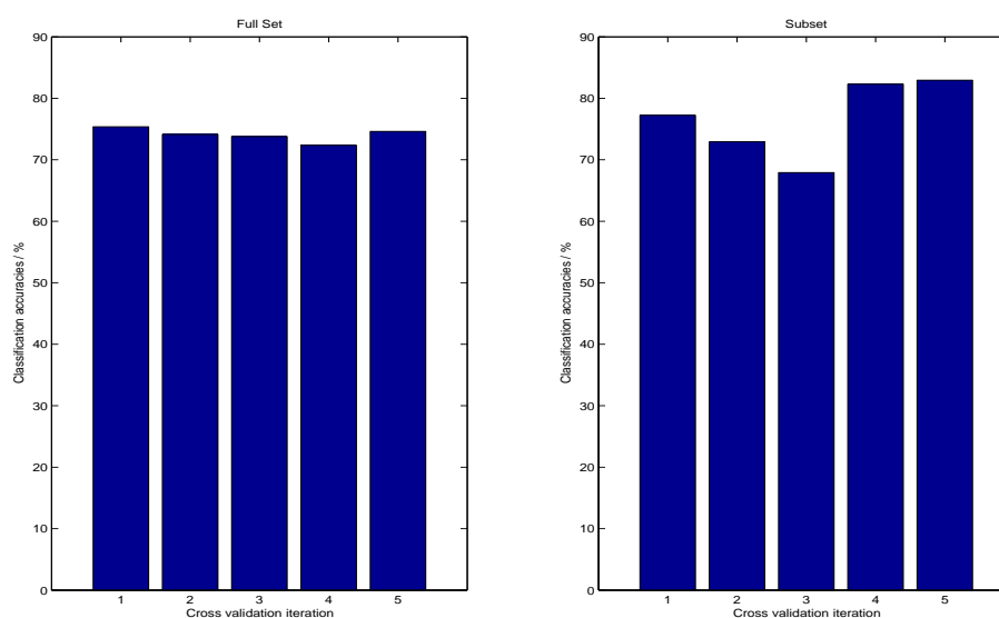
Figure 6.12. The classification accuracies on the full database 2 (left) and the subset of the database (right) that produces the results shown in table 6.6
