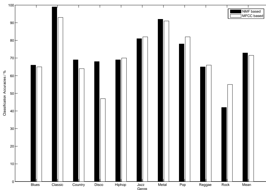
Figure 6.9. Classification accuracies on NMF and MFCC based features using a 20 component GMM
