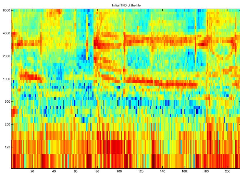
Figure 4.5. Approximation of the TFD in figure 4.3 computed with three NMF components
