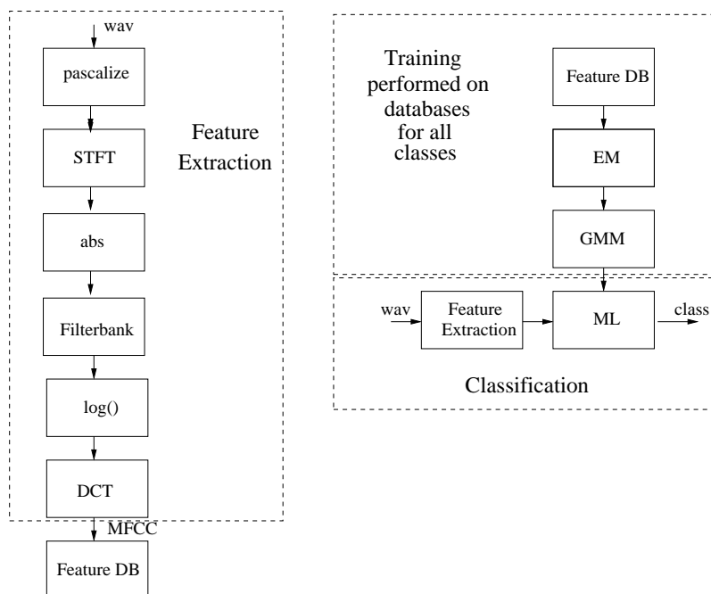
Figure 6.2. Implemented baseline system
