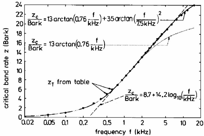
Figure 5.3. Critical bandrate z as a function of frequency f , see [50]
