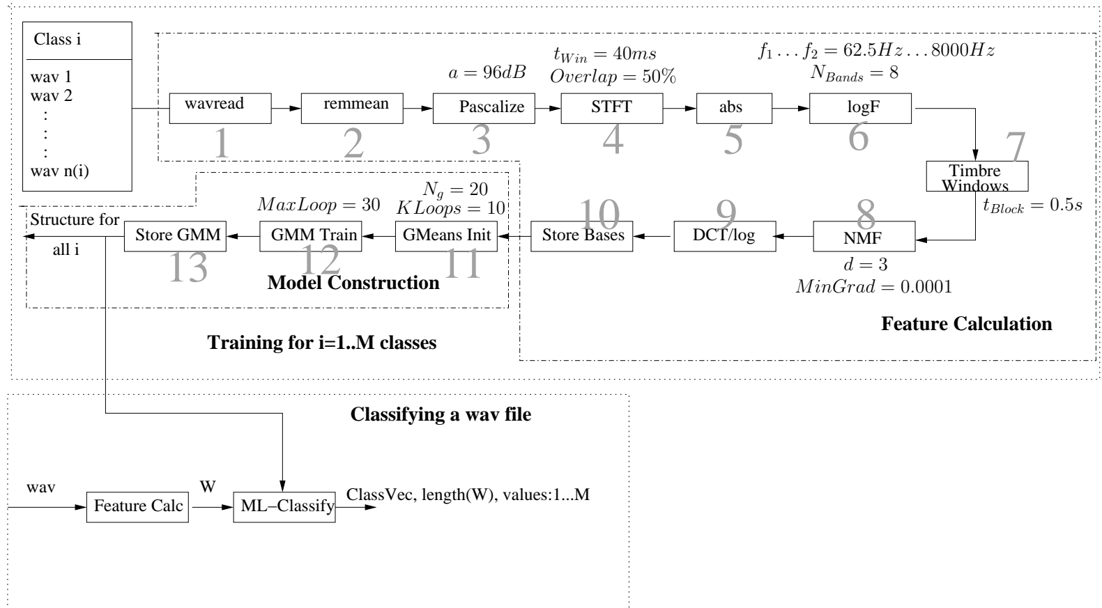
Figure 6.8. Schematic Description of the Component Based Music Similarity System
