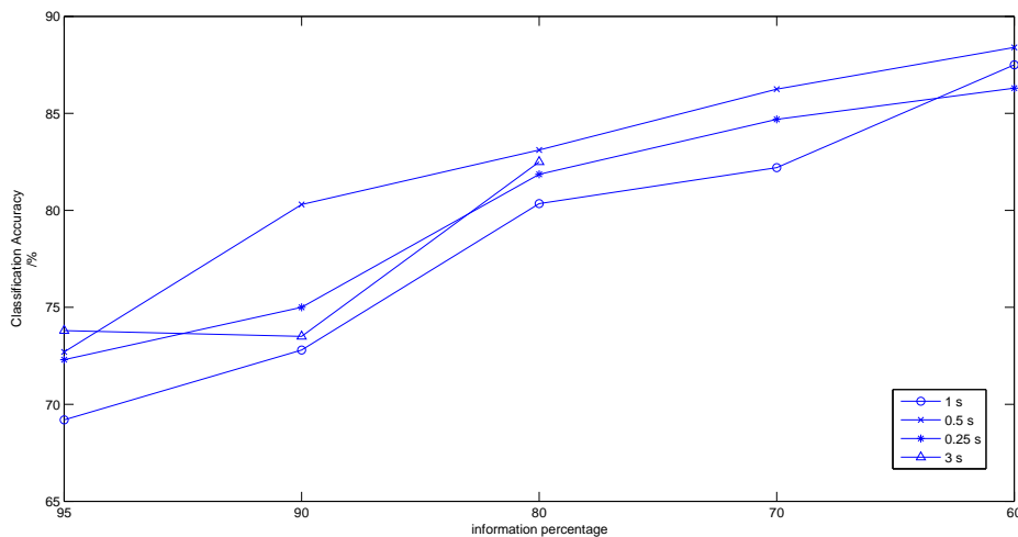
Figure 6.7. Classification accuracies for varying timbre window length and percentage of kept information
