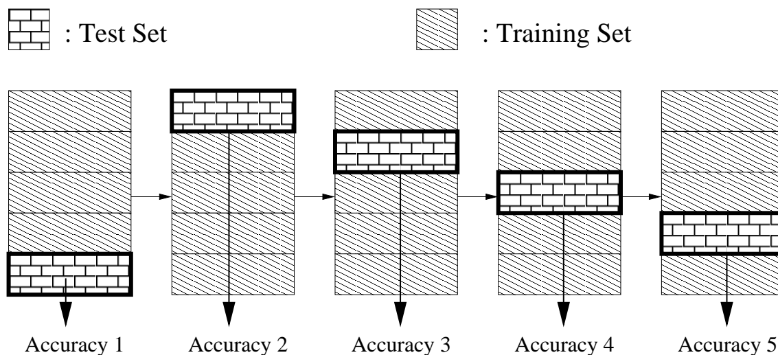
Figure 6.1. 5 fold cross validation on a data set
