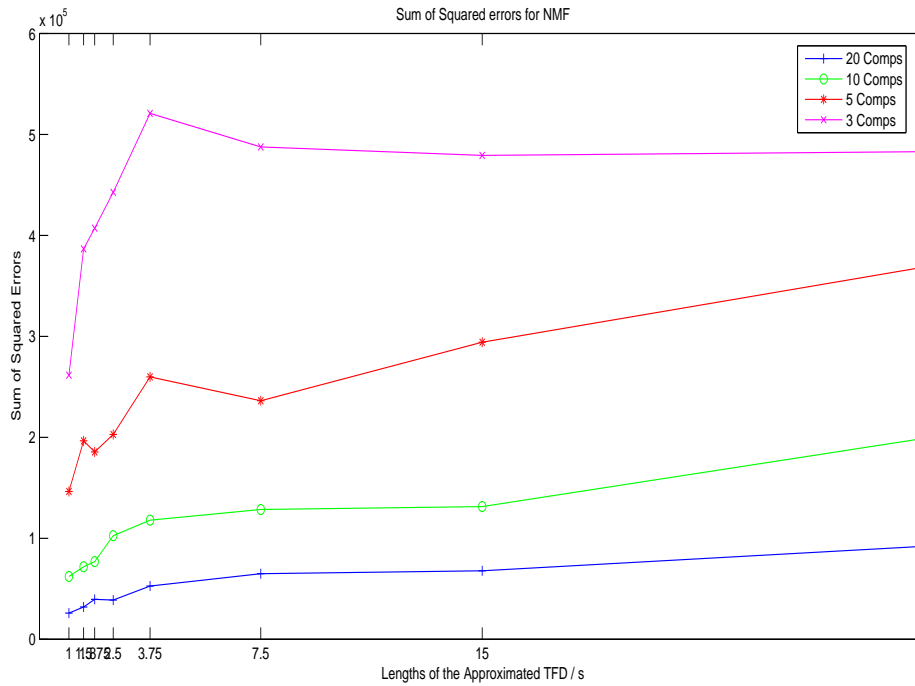
Figure 4.10. Sum of mean square errors for NMF using different number of components. The piece of music has 30 seconds length and cutting it into short pieces decreases the error.
