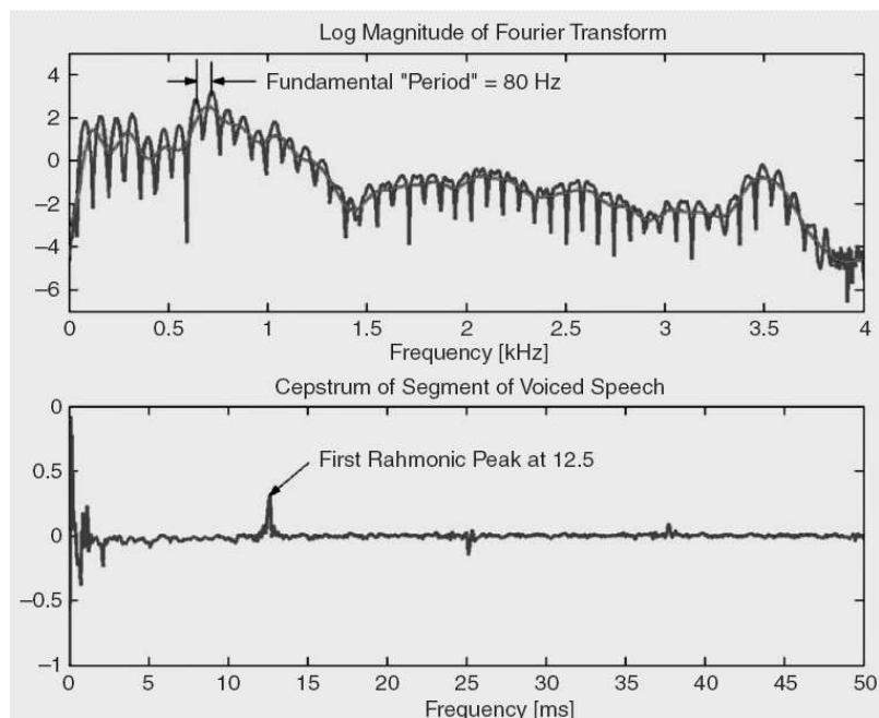
Figure 2.3. Example of liftering applied to a speech signal. The upper graph shows the unfiltered and the liftered log magnitude of the frequency spectrum. The smooth line is the liftered spectrum. As we can see in the lower graph the cepstrum before liftering has two well separated regions: the lower ones caused by the spectral envelope of the vocal tract and the higher so-called harmonics which have been caused by the excitation with a period of 80 Hz. Figure taken from [32]
