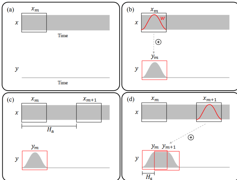
Figure 2.3: Overlap-Add method process: (a) selection of analysis frame x_m , (b) creations of synthesis frame y_m , (c) selection of analysis frame x_{m+1} (d) Overlap-add y_{m+1} to y_m - (from [3]).
