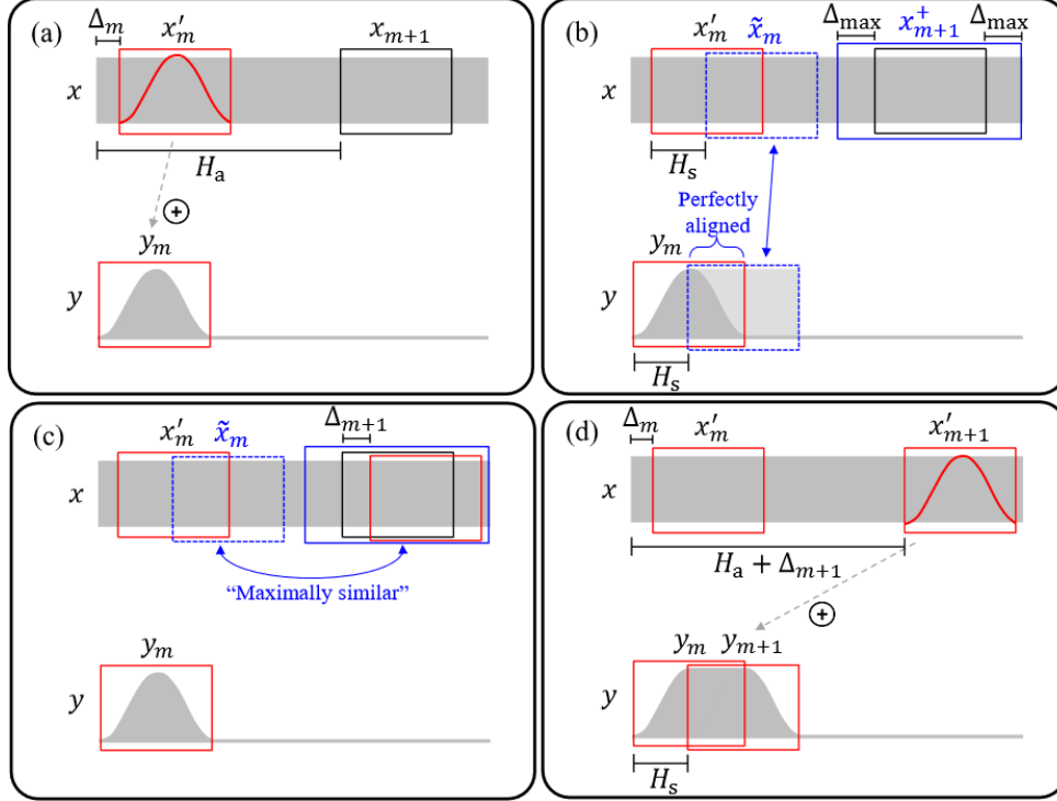
Figure 2.5: WSOLA method process : (a) adjusted analysis frame x'_m (prime symbol denotes adjustment), windowed and added to the output signal, (b,c) selection of a frame from the extended frame region x_{m+1}^+ (solid blue box) that closely matches the natural progression \tilde{x}_m (dashed blue box) of the adjusted analysis frame x'_m , (d) adjusted analysis frame x'_{m+1} for the subsequent iteration is windowed and incorporated into the output signal y - extracted from [3].
